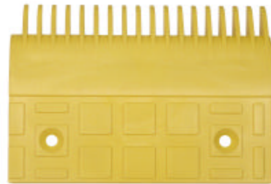
6 1/8" WIDE 18 TEETH YELLOW PLASTIC # POA453Z12Y BLACK PLASTIC # POA453Z12
